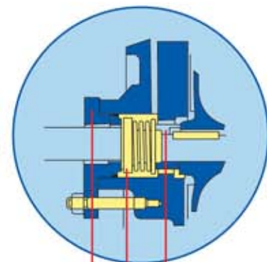
SHAFT SLEEVE MECHANICAL SEAL SEAL PLATE
