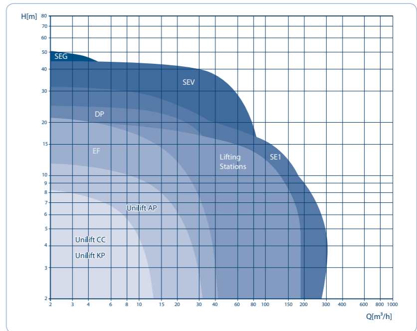
Pump performance
